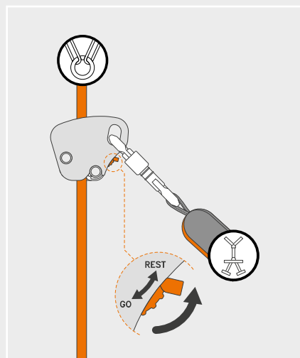
The device may be locked above the user to minimize the potential fall factor.
