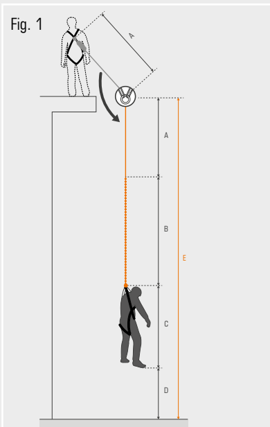
Energy absorber with integrated lanyard EN 355
