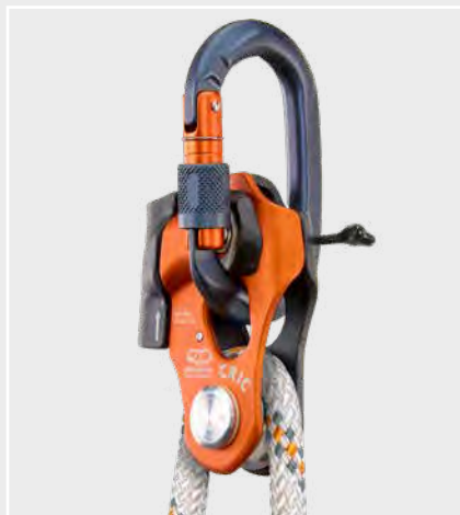
Pulley mode
